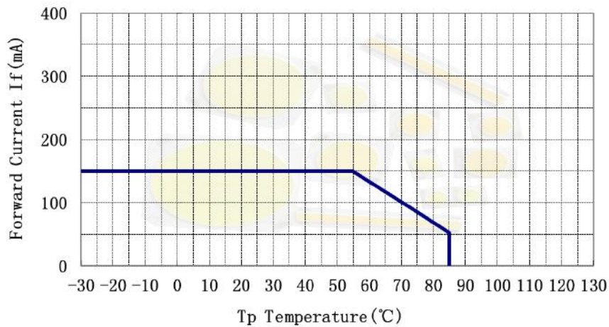
Forward Current Derating Curve
