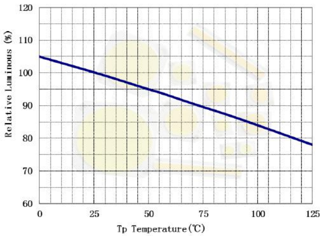
Relative Luminous(@30mA)VS. Tp Temperature
