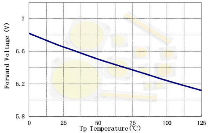
Forward Voltage(@30mA)VS. Tp Temperature
